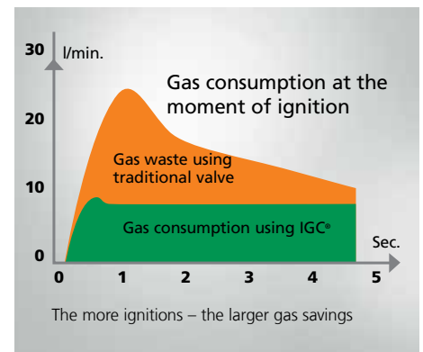
IGC® Intelligent Gas Control Synergic gas regulation saves gas every time the weld pool is established.
